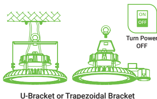
U-Bracket or Trapezoidal Bracket
