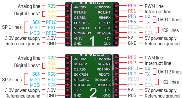
Figure 9-1: mikroBUS™ individual and shared lines
