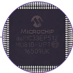
Figure 3-1: dsPIC33EP512MU810 microcontroller
