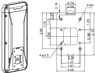
Figure3-3 Dimensions (Unit: inch)
