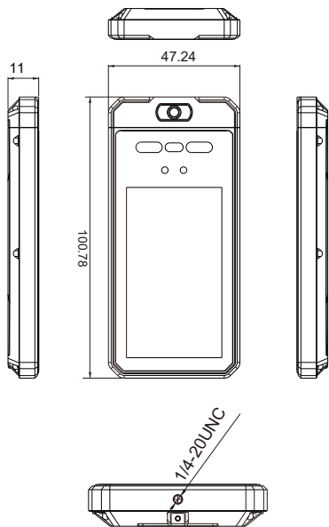
Figure 2-3Dimensions (Unit: inch)
