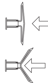
Fig. 3 Wall Anchor
