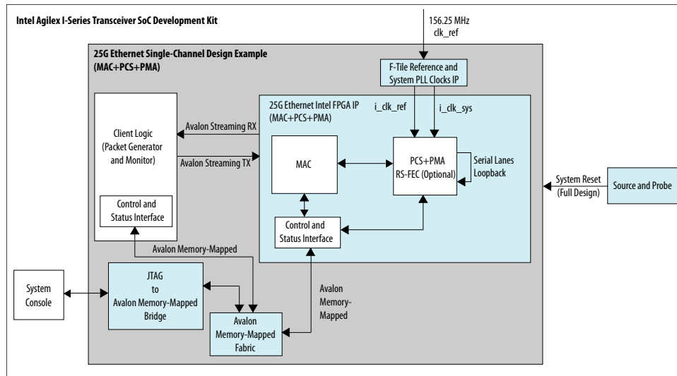
Figure 5. Block Diagram—F-tile 25G Ethernet Design Example (MAC+PCS+PMA Core Variant)
