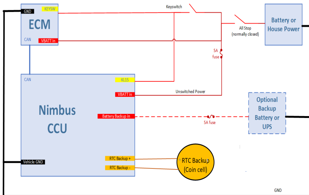
Figure 4 Grounding Scheme
