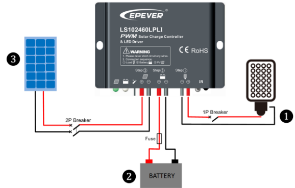
Figure 2 Wiring
