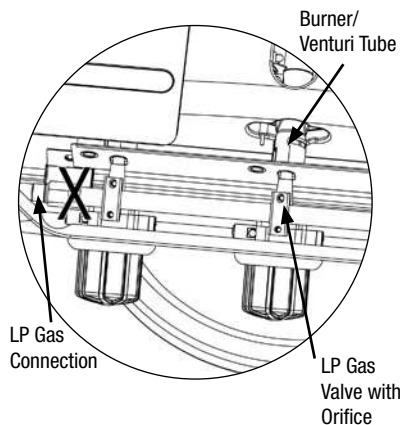
Figure 1: Main Burners
