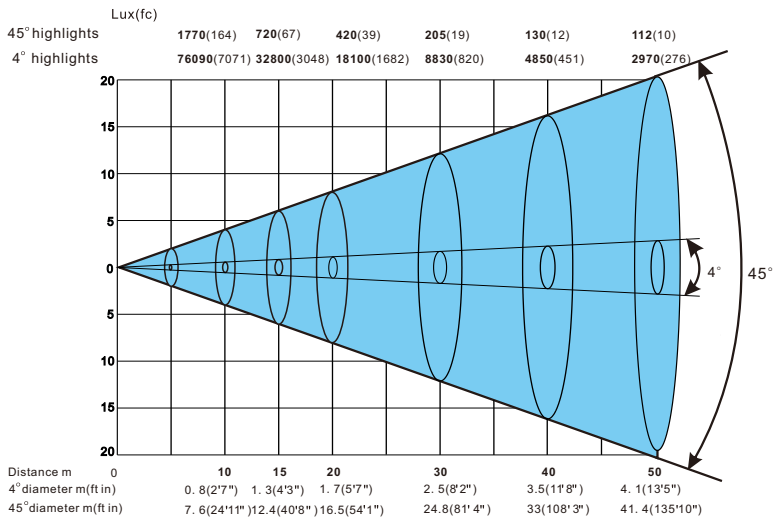
射距、光斑直径与照度关系图(BEAM模式) distance, spot diameter and illumination diagram (Beam model)
