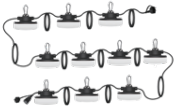
STRING-100
