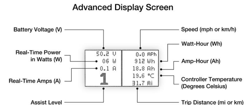
Fig. 24 - Data on the Advanced Display Screen
