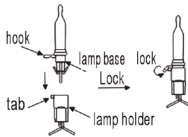
Fig. 2 Replace with the spare lamp
