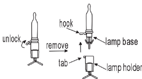
Fig. 1 Unlock and remove the burned out lamp
