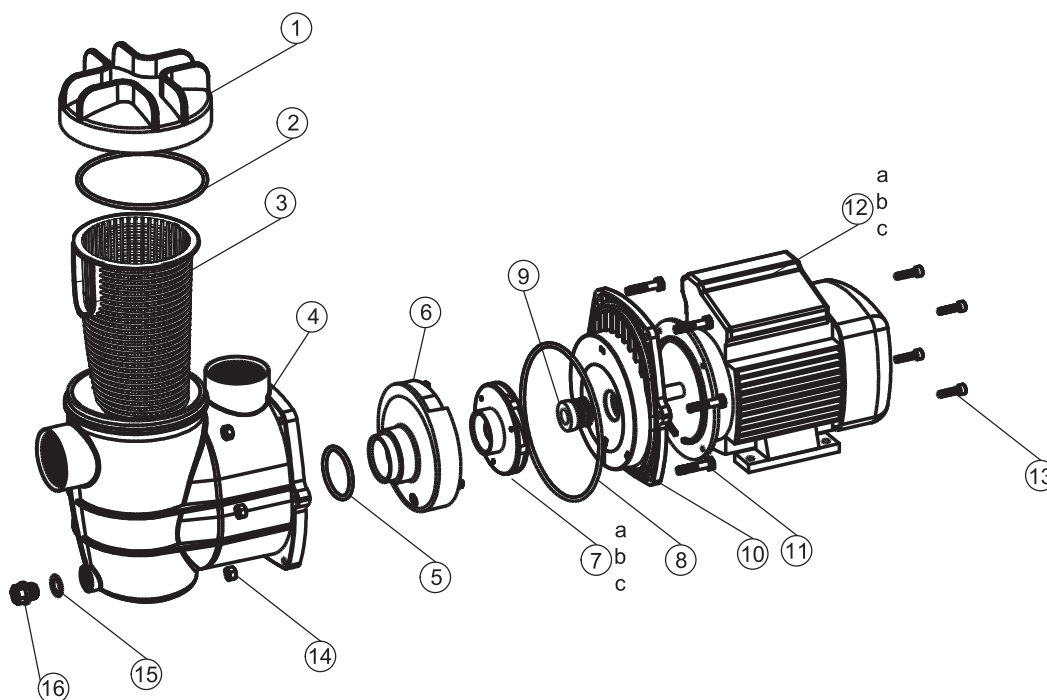
71236/714061 PUMP MODELS
