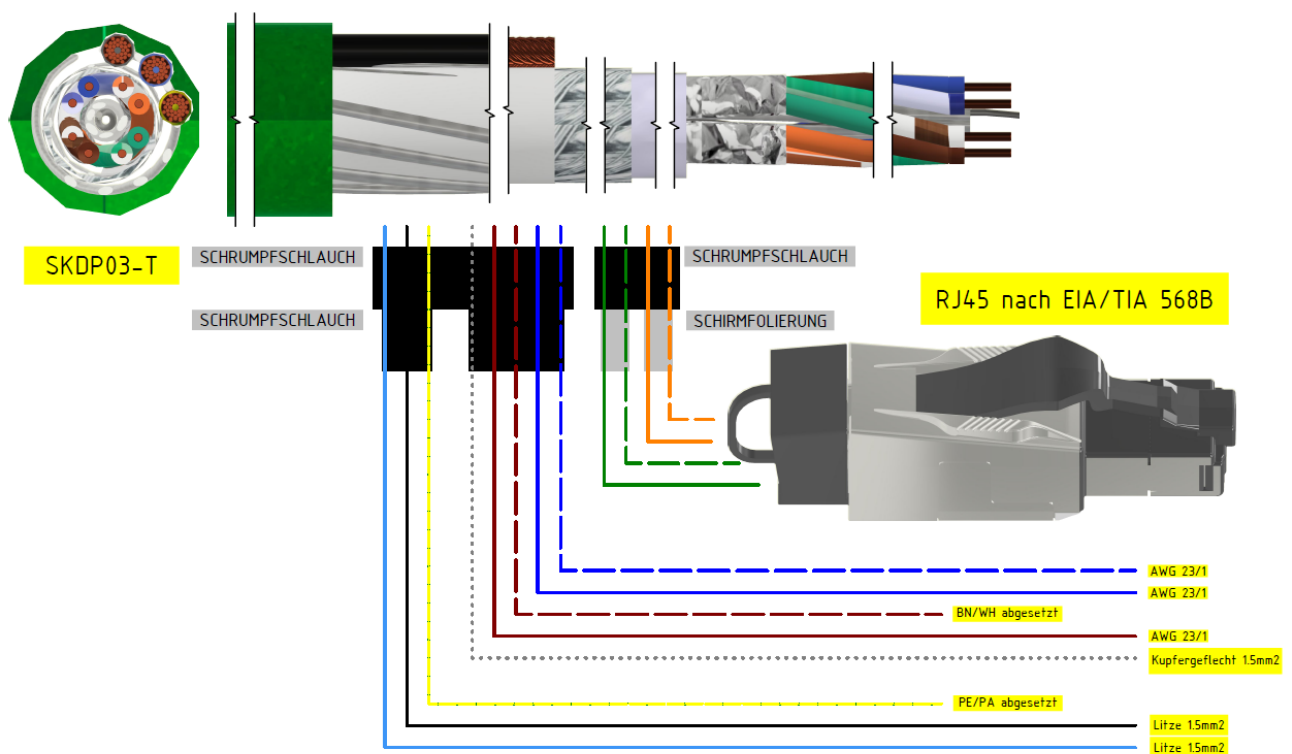
Figure 5-8 Plug assignment RJ45
