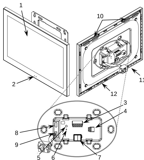
Figure 2 Schematic diagram (Z50)
