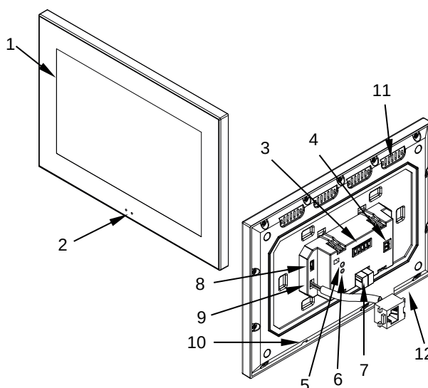
Figure 1 Schematic diagram (Z50)
