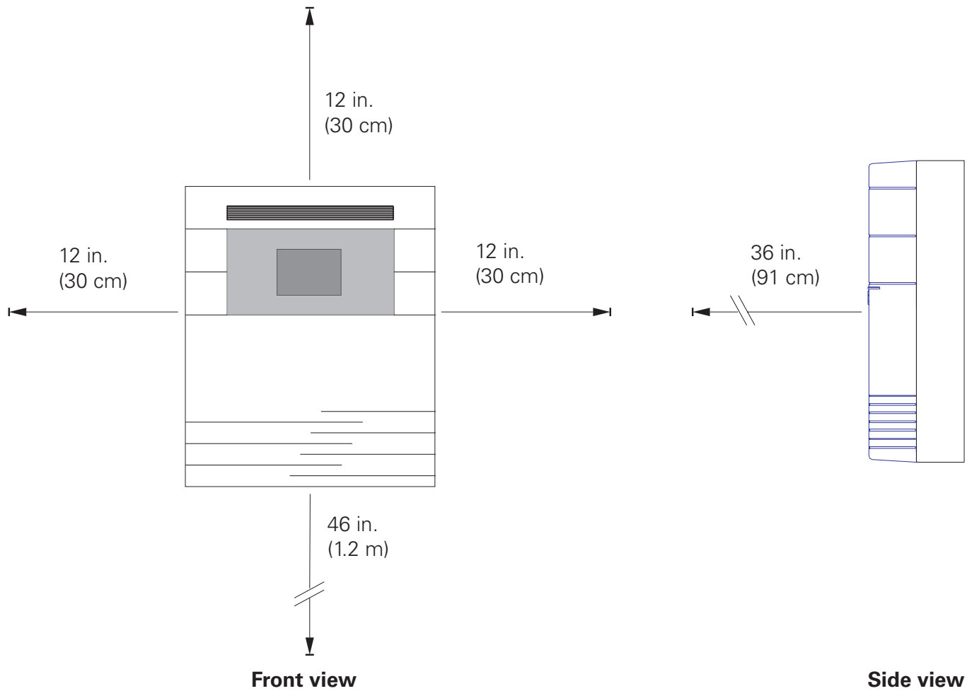
Figure 9. BCU clearances
