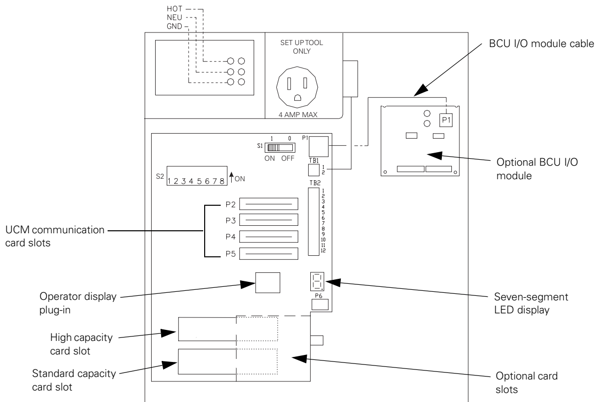
Figure 5. BCU housing and component layout
