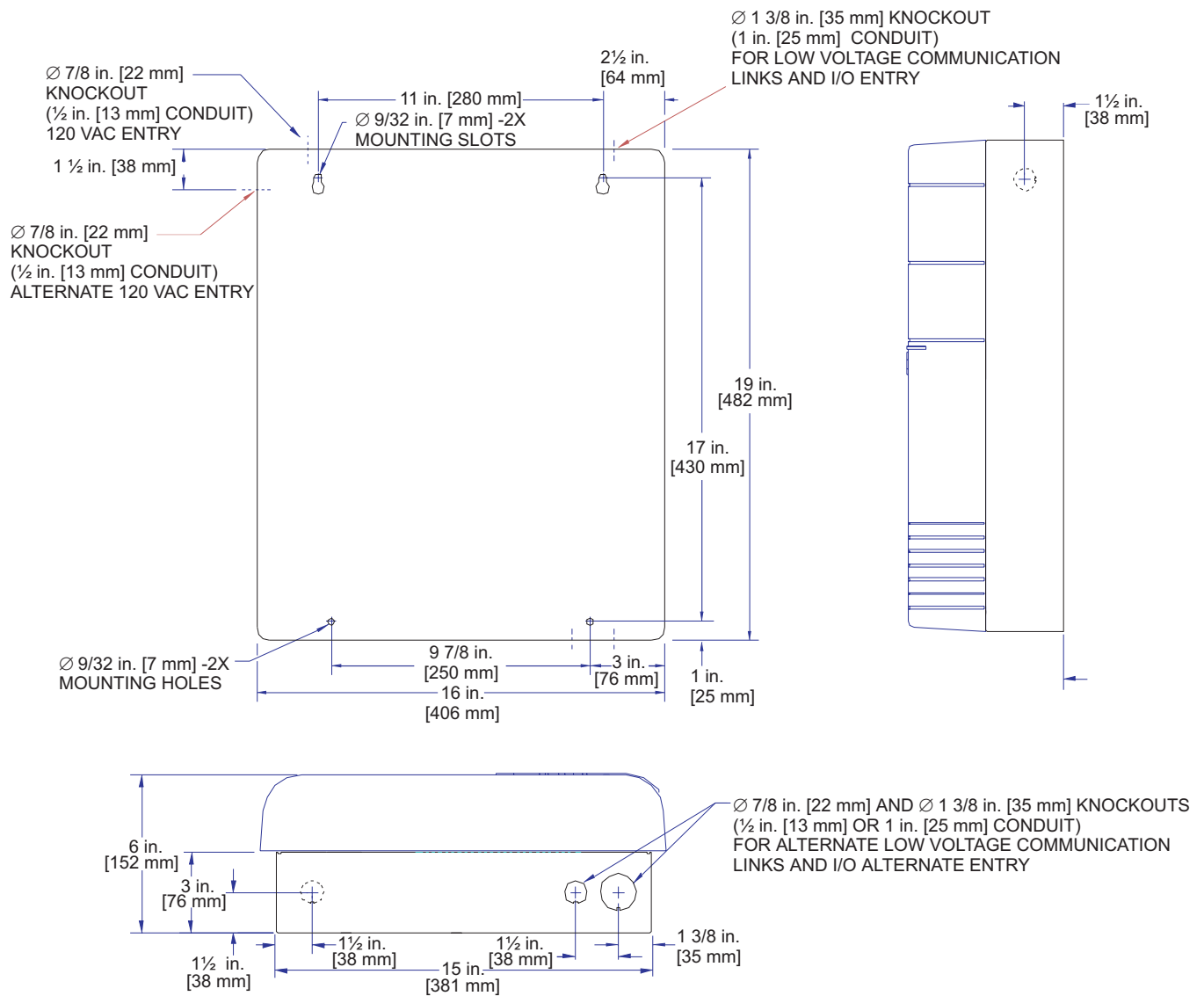
Figure 8. BCU dimensions and cable access
