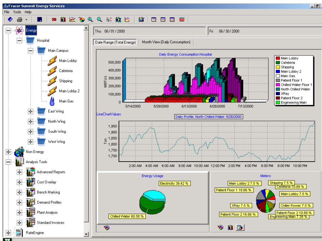
Figure 6. Example of Tracer Summit Energy Services software
