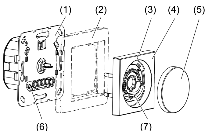
Image 1: Device components
