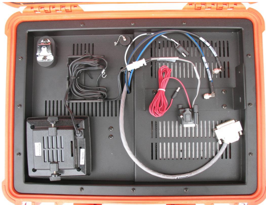
Figure 6 Mounting the Mobile speaker- O3 Control Head Model
