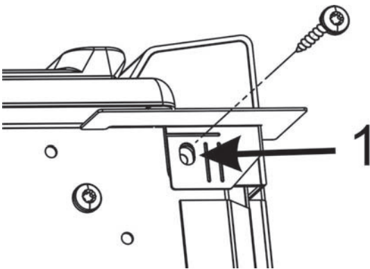
Figure 4: Screw placement
