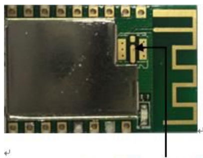
Figure 2-6 On-board antenna
