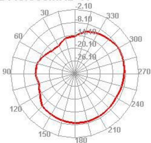
Figure 2-7 Antenna pattern
