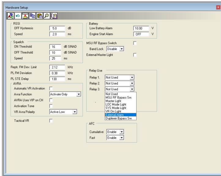
Figure 17 - Relay Use options
