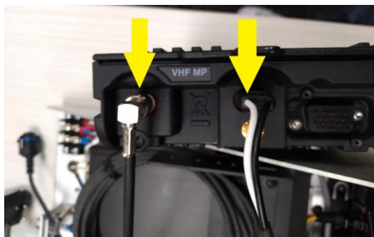
Figure 9 - DC and RF cable connections
