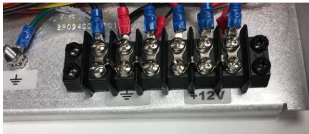
Figure 12 - DC Power connections
