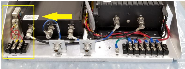
Figure 15 - Optional external alarm hardware location
