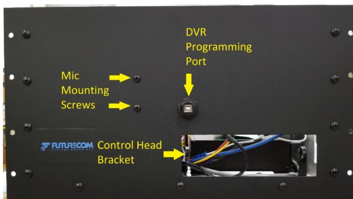
Figure 2 - Rackmount DVRS - As Received (front view)
