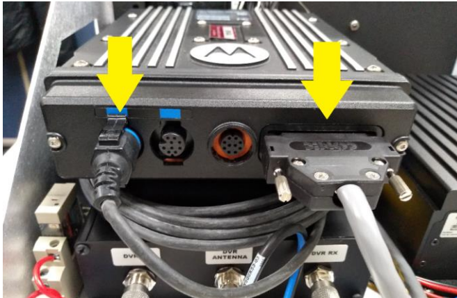
Figure 11 - Installation of the MSU – step 2
