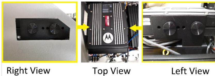
Figure 10 - Installation of the MSU – step 1
