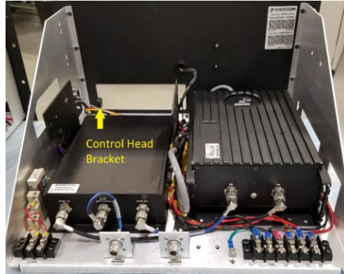
Figure 3 - Rackmount DVRS - As Received (rear view)
