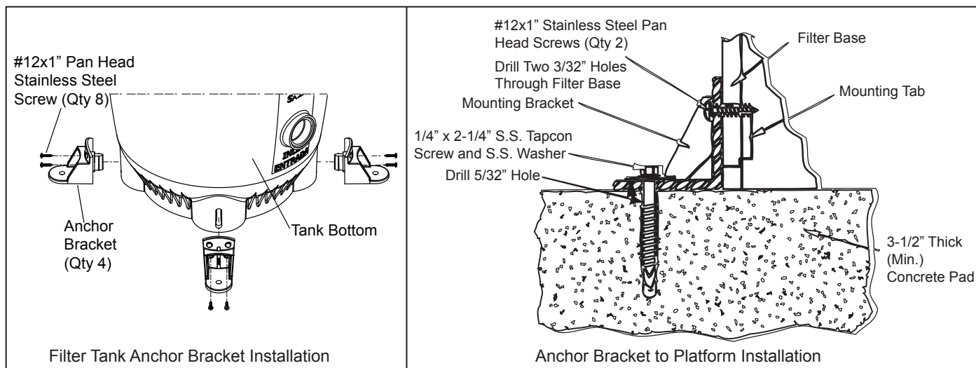
Figure 3. Anchor Bracket Installation
