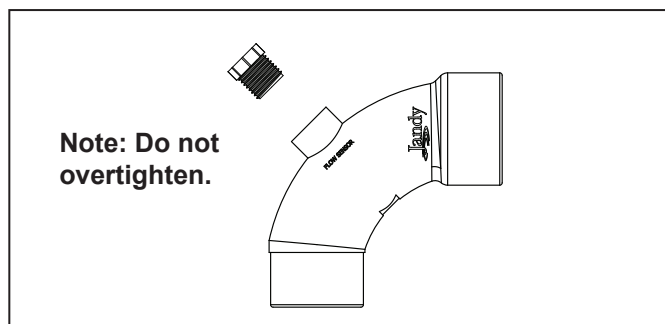
Figure 7. Sweep Elbow
