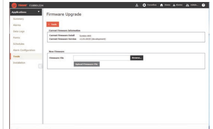
Figure 4. Select firmware
