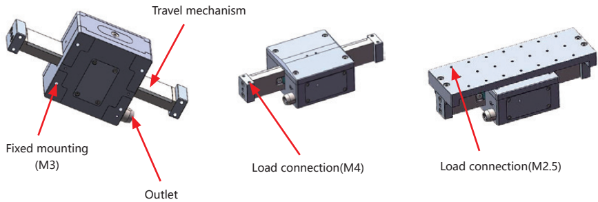
N31 Installation diagram
