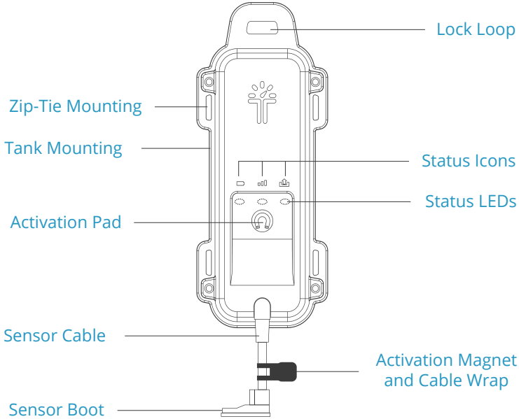
Tank Monitor
