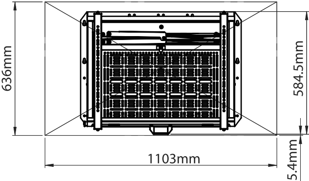
49" SCREEN - CLOSE
