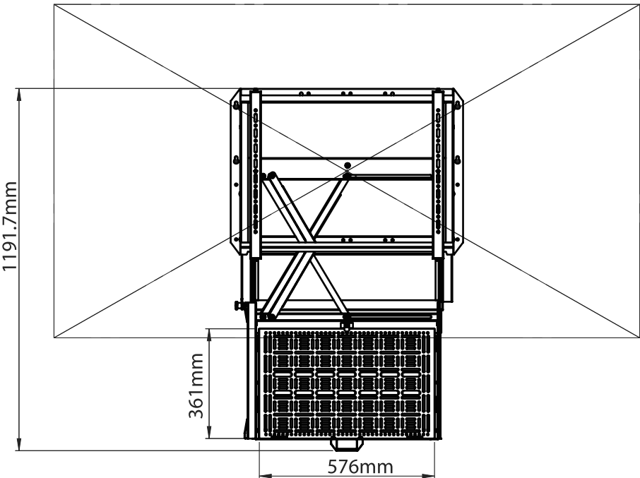
86" SCREEN - OPEN
