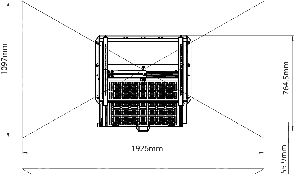
86" SCREEN - CLOSE
