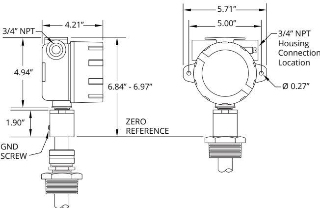
MPX-R Housing Dimensions
