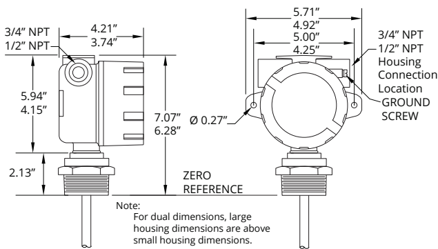
MPX-E Chemical Housing Dimensions
