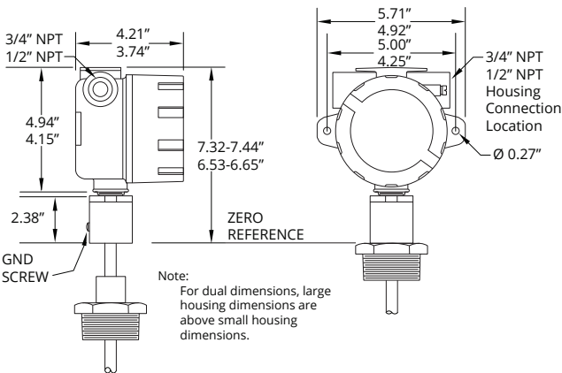
MPX-E Housing Dimensions
