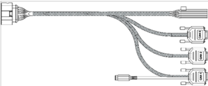
Figure 2. CLM 3600 Starter Cable
