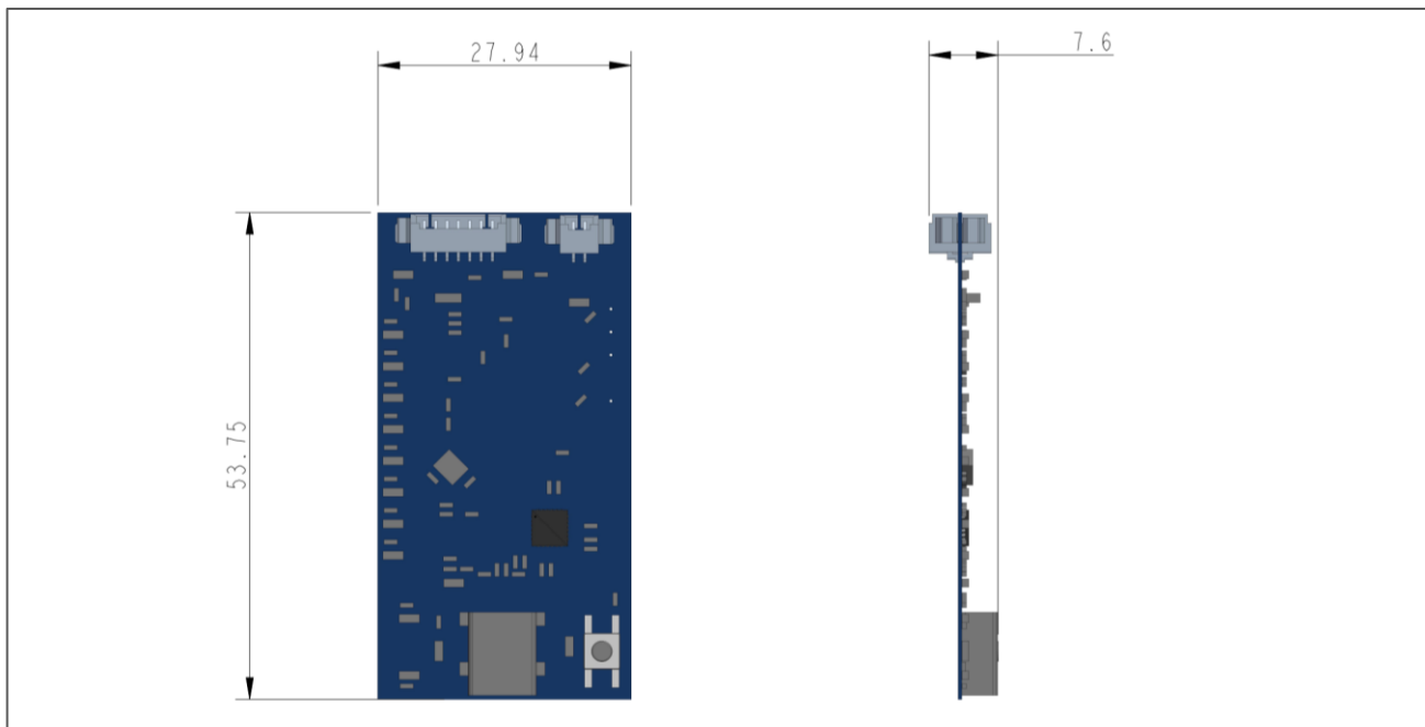
Figure 2 TTL / CAN to USB converter dimension schematic. Unit: mm
