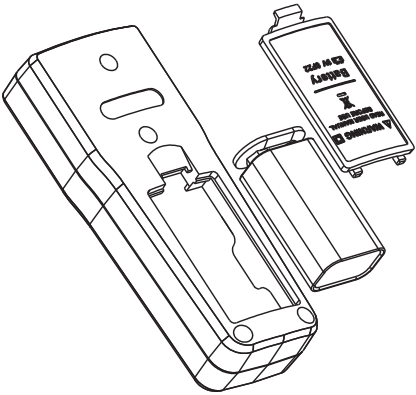
Figure 4 UT682 Transmitter
