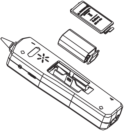
Figure 5 UT682 Receiver
