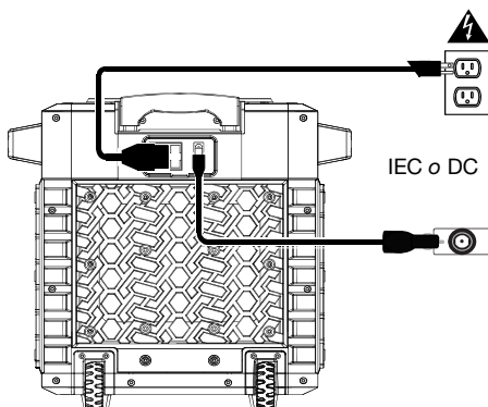
Panel trasero
