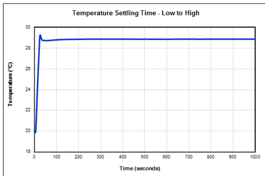
Figure 8 Typical Heating Response
