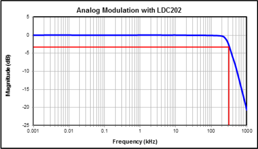
Figure 10 Low Frequency Modulation Through LD Controller
