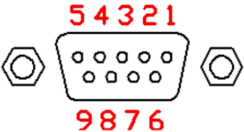
Figure 4 LD Controller DB9 Connection
