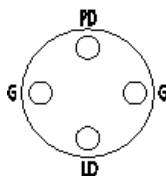
Figure 3 Laser Diode Socket
