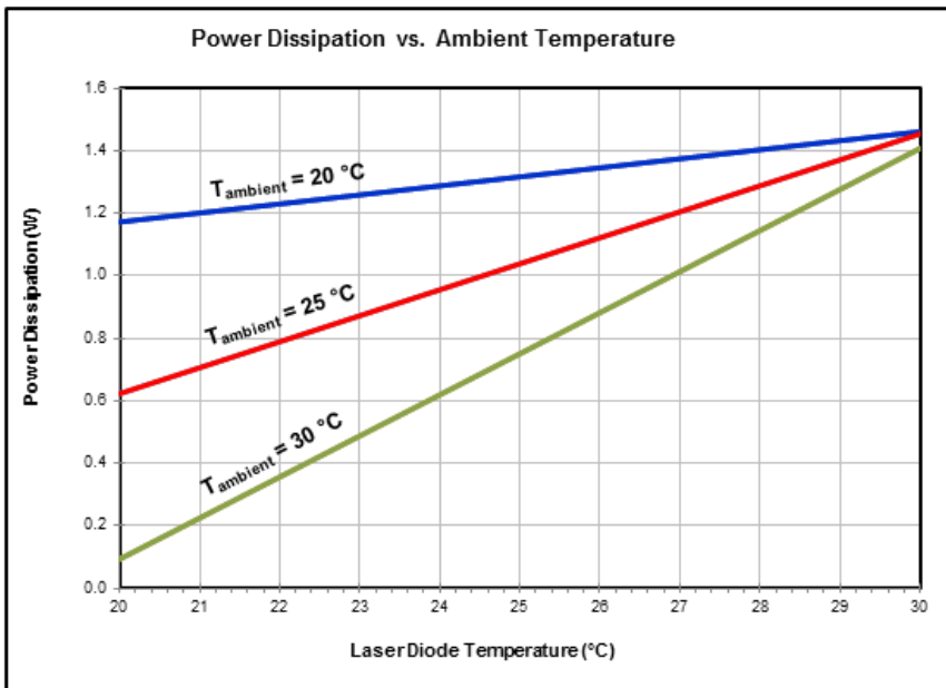
Figure 6 Power Dissipation vs. Ambient Temperature
