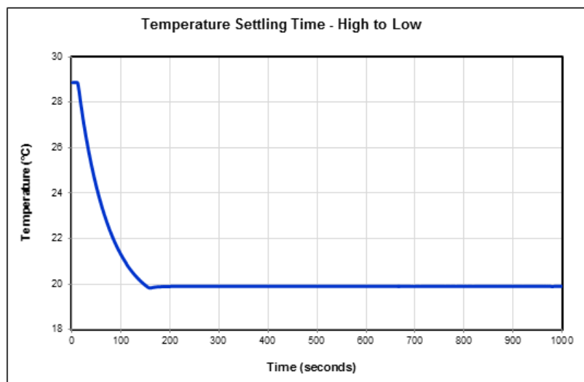
Figure 9 Typical Cooling Response
