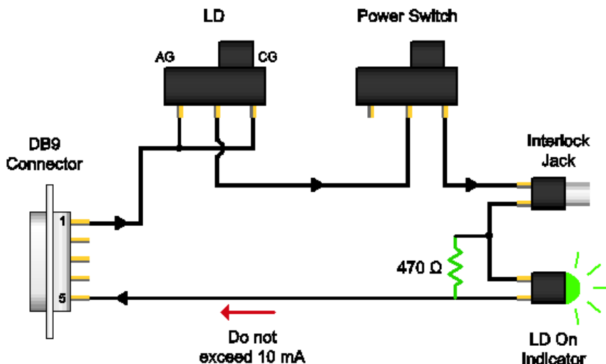
Figure 5 Interlock Connection Schematic
