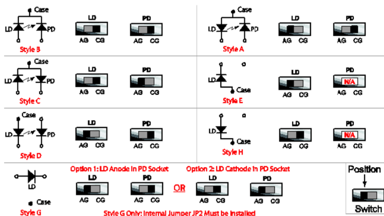
Figure 2 Polarity Switch Settings
