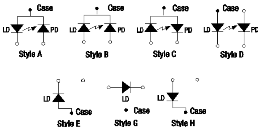
Figure 1 Supported Pin Configurations
