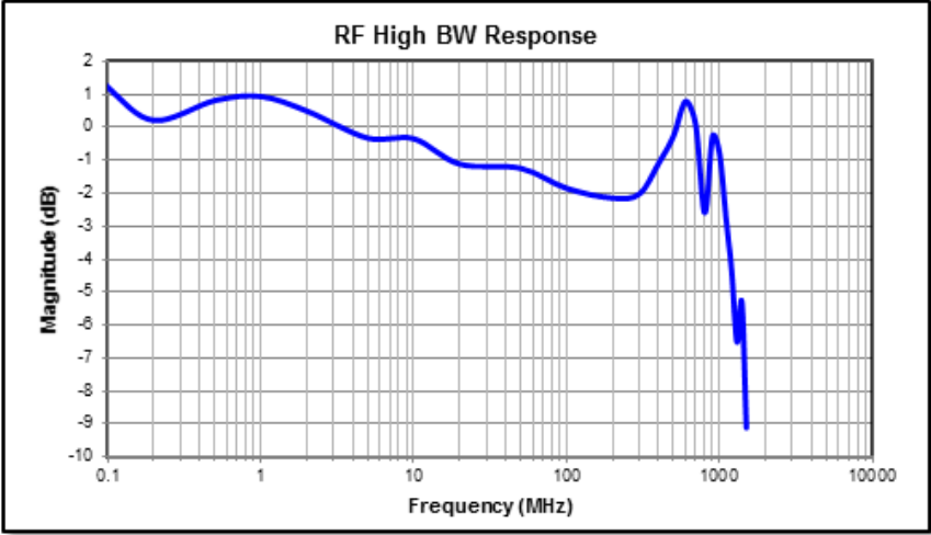
Figure 11 RF Modulation Through SMA Connector on LM9LP
