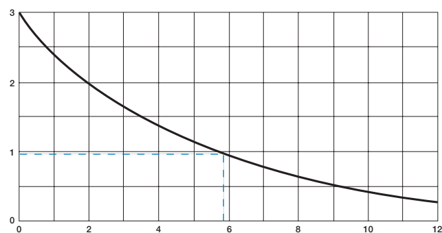
Diagram 2, addition of sound levels.
