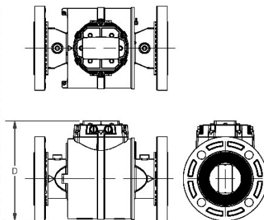
ANSI FLANGE WITH QB ELECTRONICS
