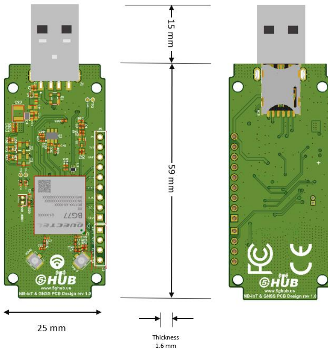
Figure 3. Physical Characteristics.
