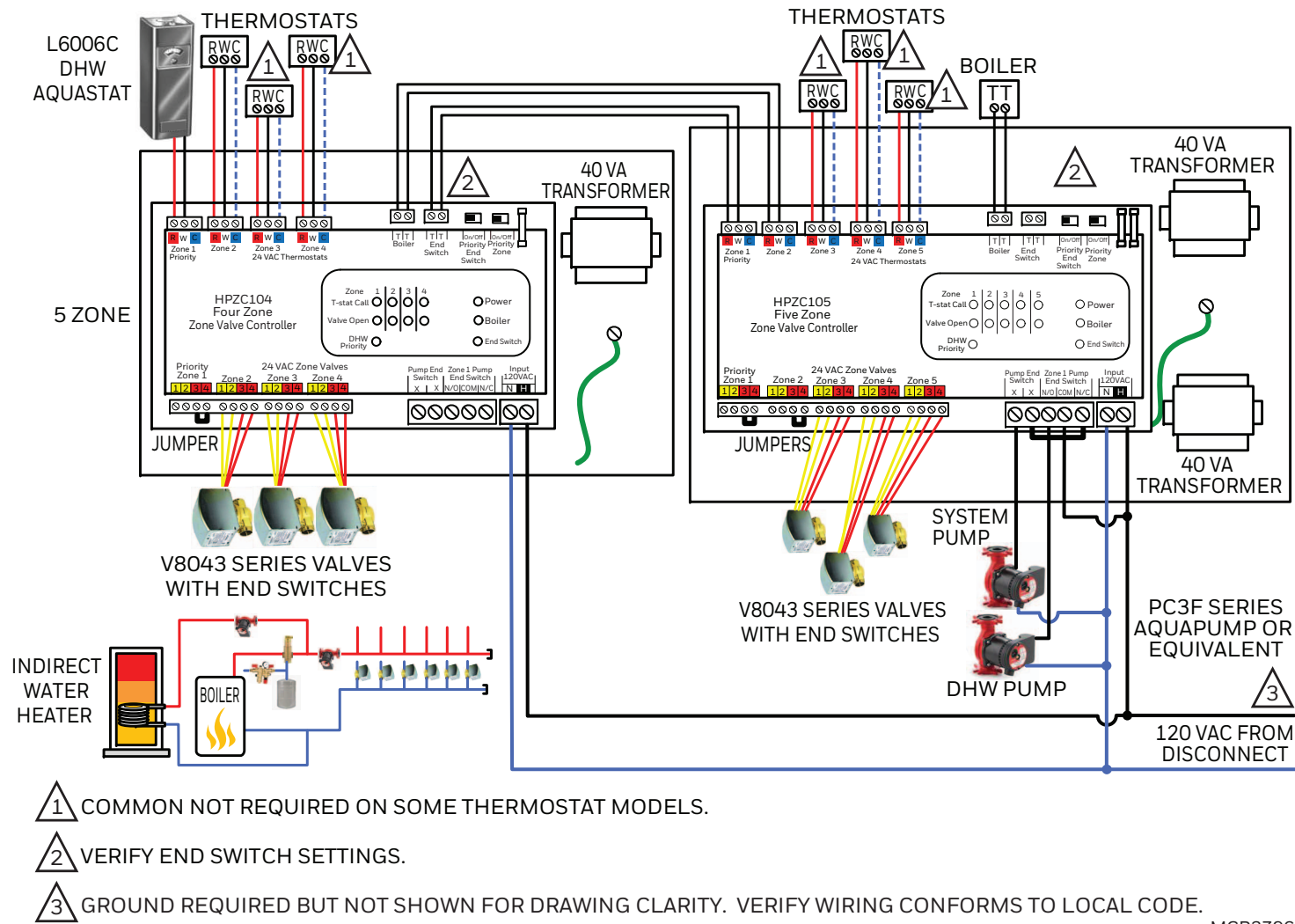
Fig. 2. More than 6 zone valves when DHW priority is desired. (DHW is considered one of the zones).
