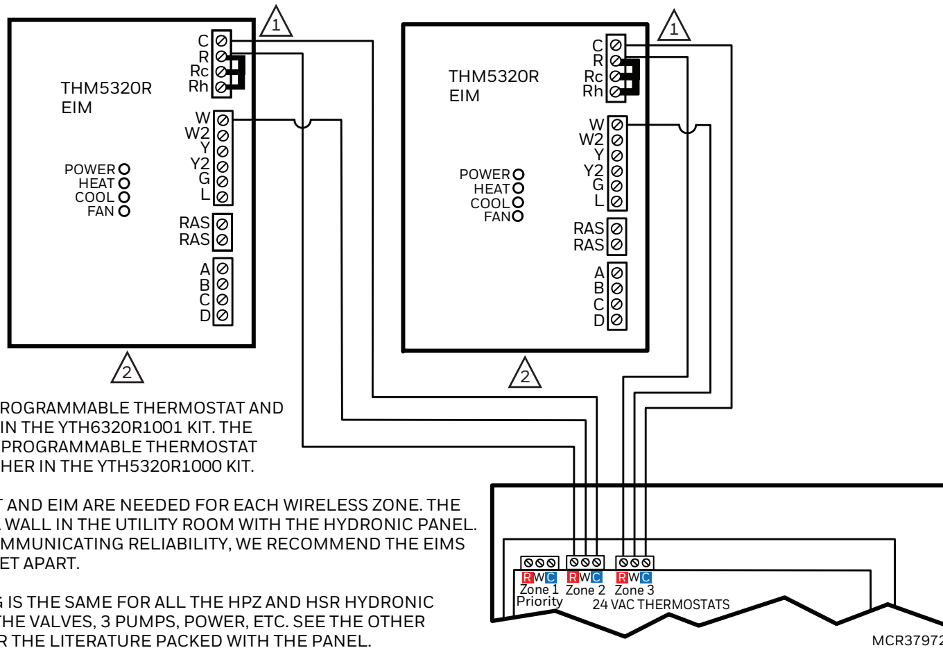
Fig. 7. Wireless FocusPRO thermostats with Hydronic panels.
