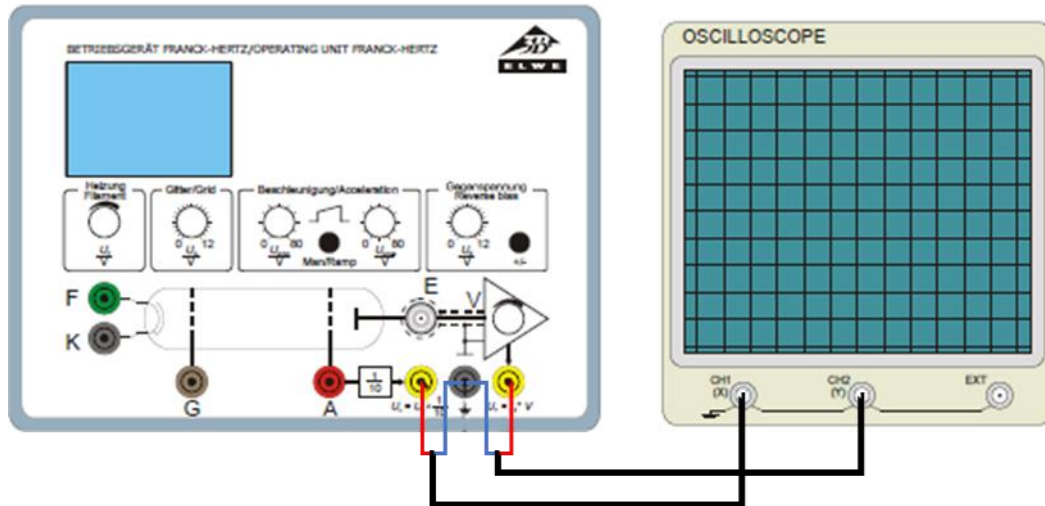
Fig. 3: Electrical connection of an oscilloscope to the Franck-Hertz power supply
