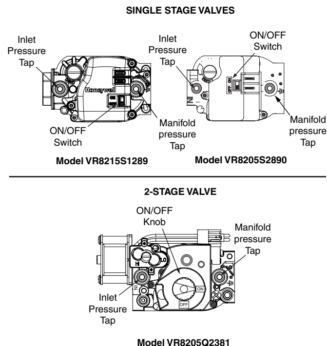
Figure 5. Inlet & Manifold Pressure Tap Locations
