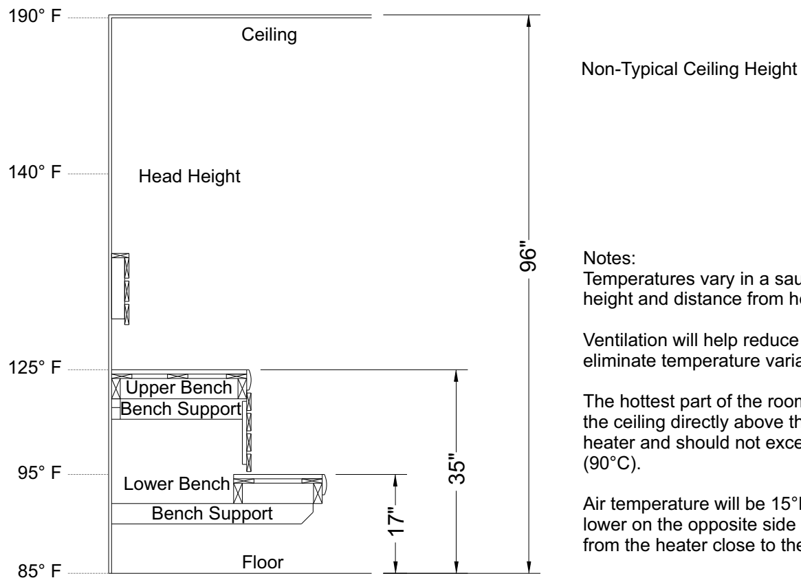
DIAGRAM 12: ROOM TEMPERATURES
