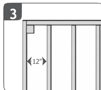
Diagonal (45 degree) Installation Substructure 12" on center maximum joists. Different angles will require – 60 degrees 14" on center spacing, 30 degrees 6" on center
