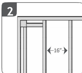
Picture Frame-Perpendicular Installation Substructure 16" on center maximum joists plus additional support for picture frame structure. (12" on center for commercial applications.)
