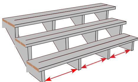
Picture Frame-Perpendicular Installation Substructure 16" on center maximum joists plus additional support for picture frame structure. (12" on center for commercial applications.)
