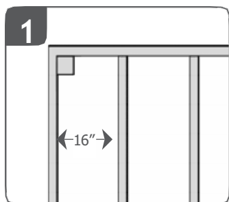
Perpendicular Installation Substructure 16" on center maximum joists. (12" on center for commercial applications.)
