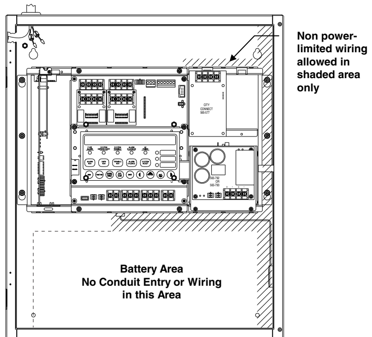
Figure 8. Wiring Information
