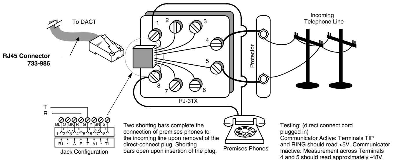
Figure 4. Telephone Company Wiring
