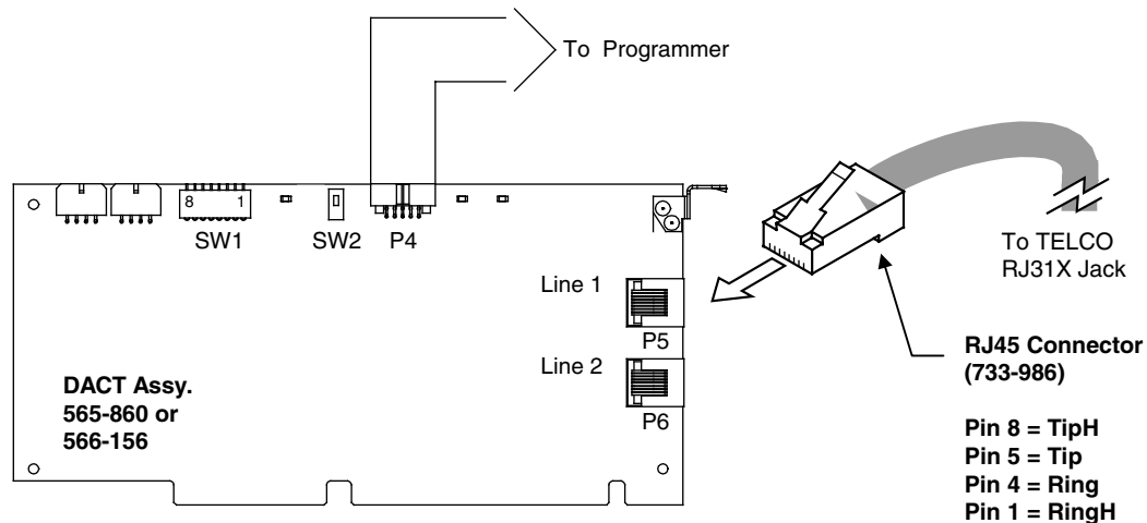
Figure 2. 4010-9810 Common Event Reporting DACT (742-155)
