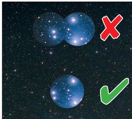
Astronomical observations
