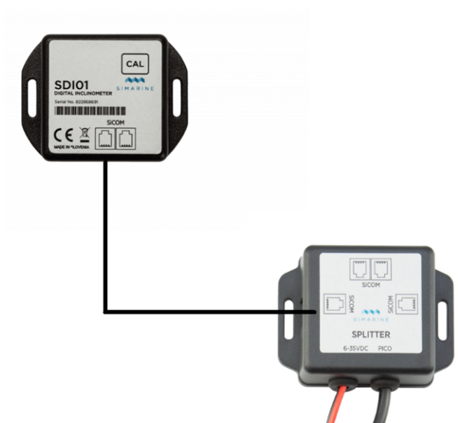
STANDARD WIRING – DIRECTLY TO THE SPLITTER
