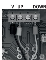
Connecting terminals for external buttons
