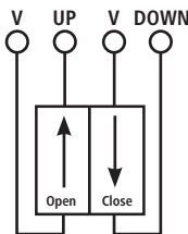
Connecting terminals for external buttons
