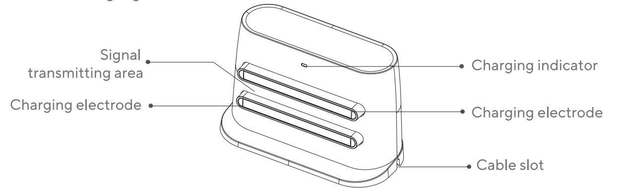
Charging Dock
