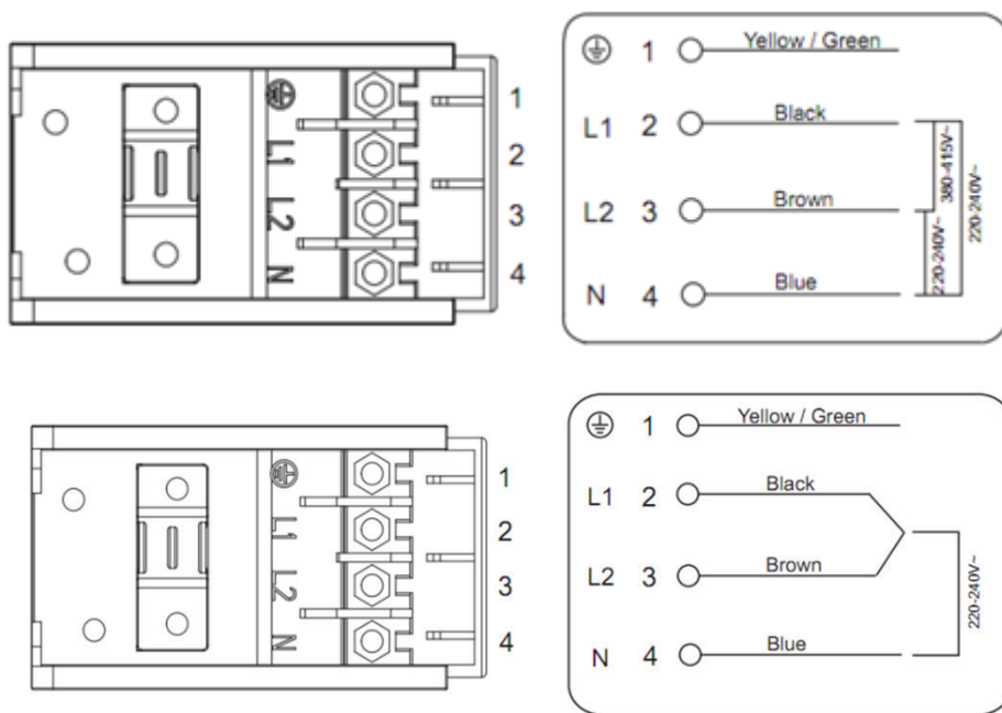
Wiring Diagram
