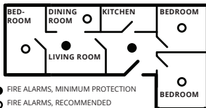
MULTI-STOREY BUILDING WITH MULTIPLE BEDROOMS
