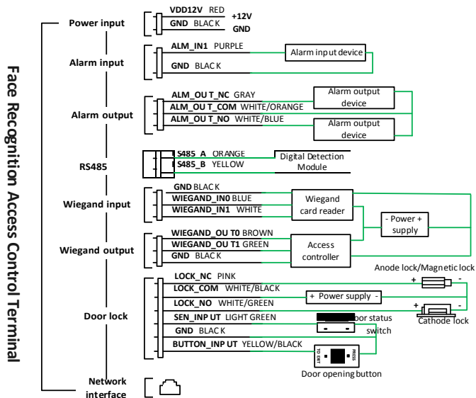
Figure 3-1 Wiring Schematic Diagrams (without Security Module)
