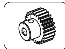
No. 505126 3,17mm Pignon moteur 22Z 48DP Motor gear 22T 48DP
