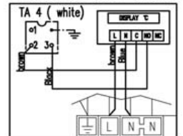
Electronic thermostat : OPTIONAL
