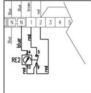
OPTIONAL - delay starting relay
